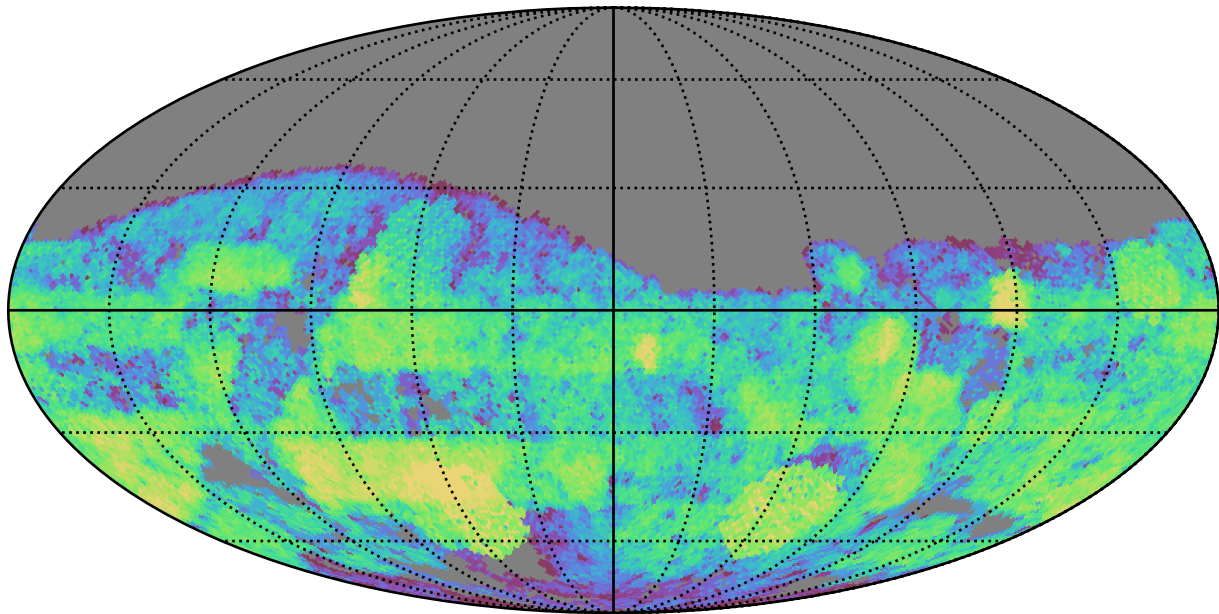
too_combined_s0.5_v3.4_10yrs Yr 3-4 g band: CoaddM5
