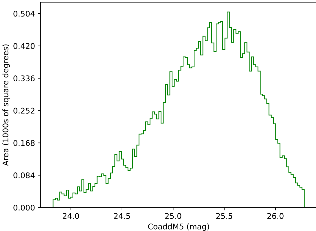
too_combined_s0.5_v3.4_10yrs Yr 3-4 g band: CoaddM5
