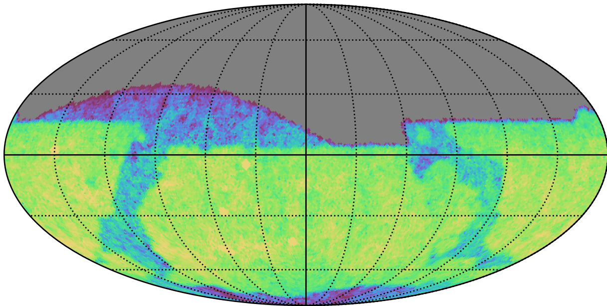
too_combined_s0.5_v3.4_10yrs Yr 1 z band: CoaddM5
