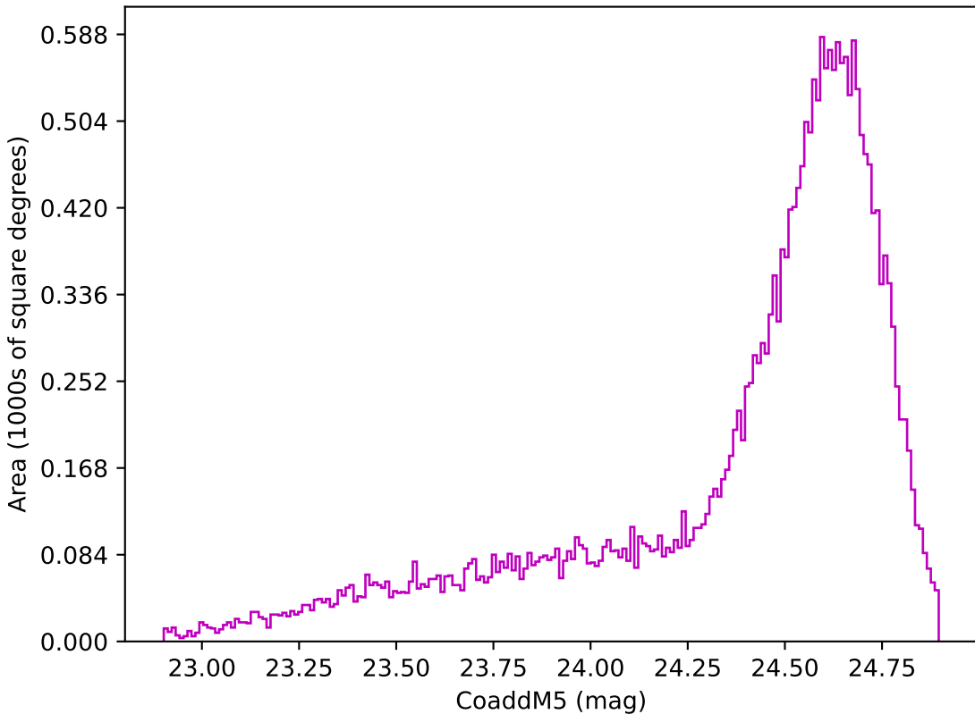
too_combined_s0.5_v3.4_10yrs Yr 1 z band: CoaddM5
