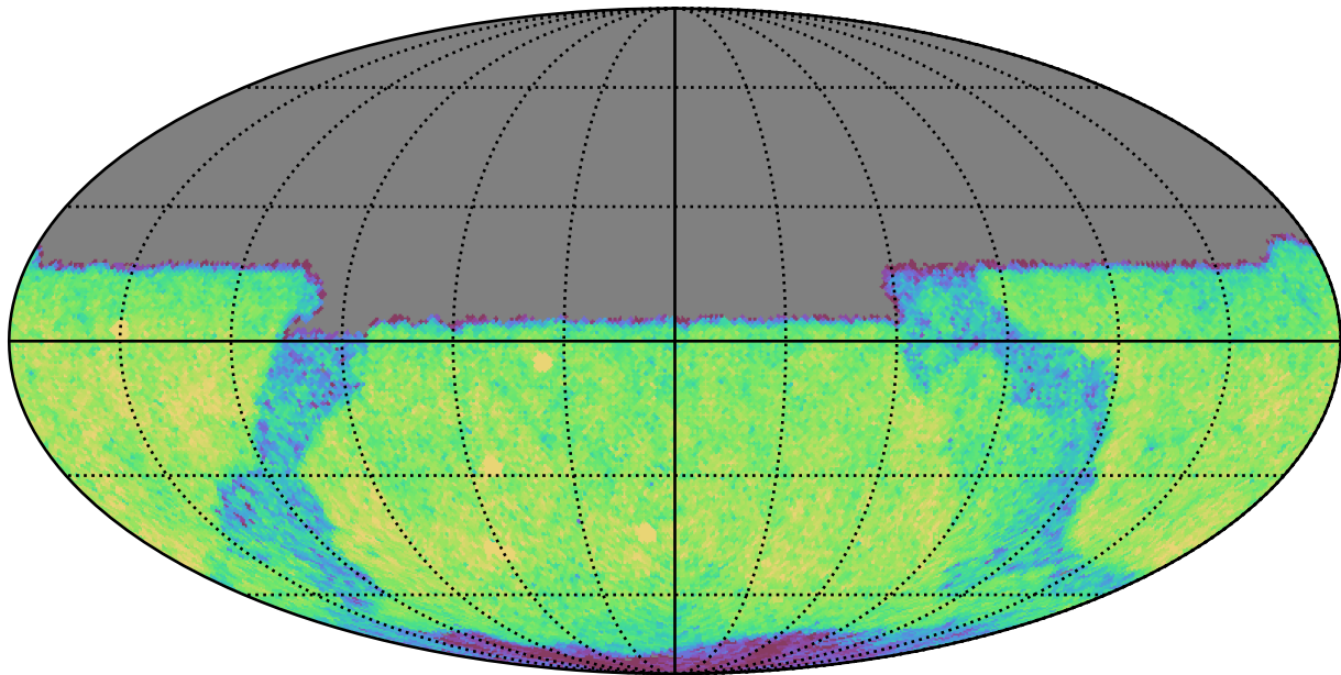
too_combined_s0.5_v3.4_10yrs Yr 1 y band: CoaddM5
