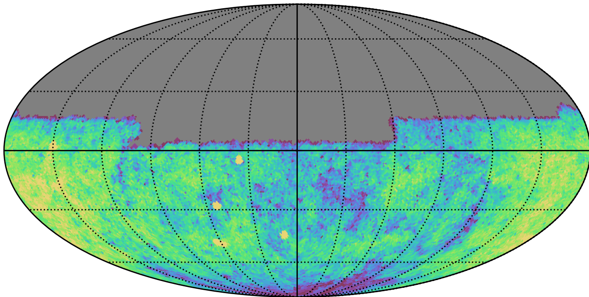
too_combined_s0.5_v3.4_10yrs Yr 1 u band: CoaddM5
