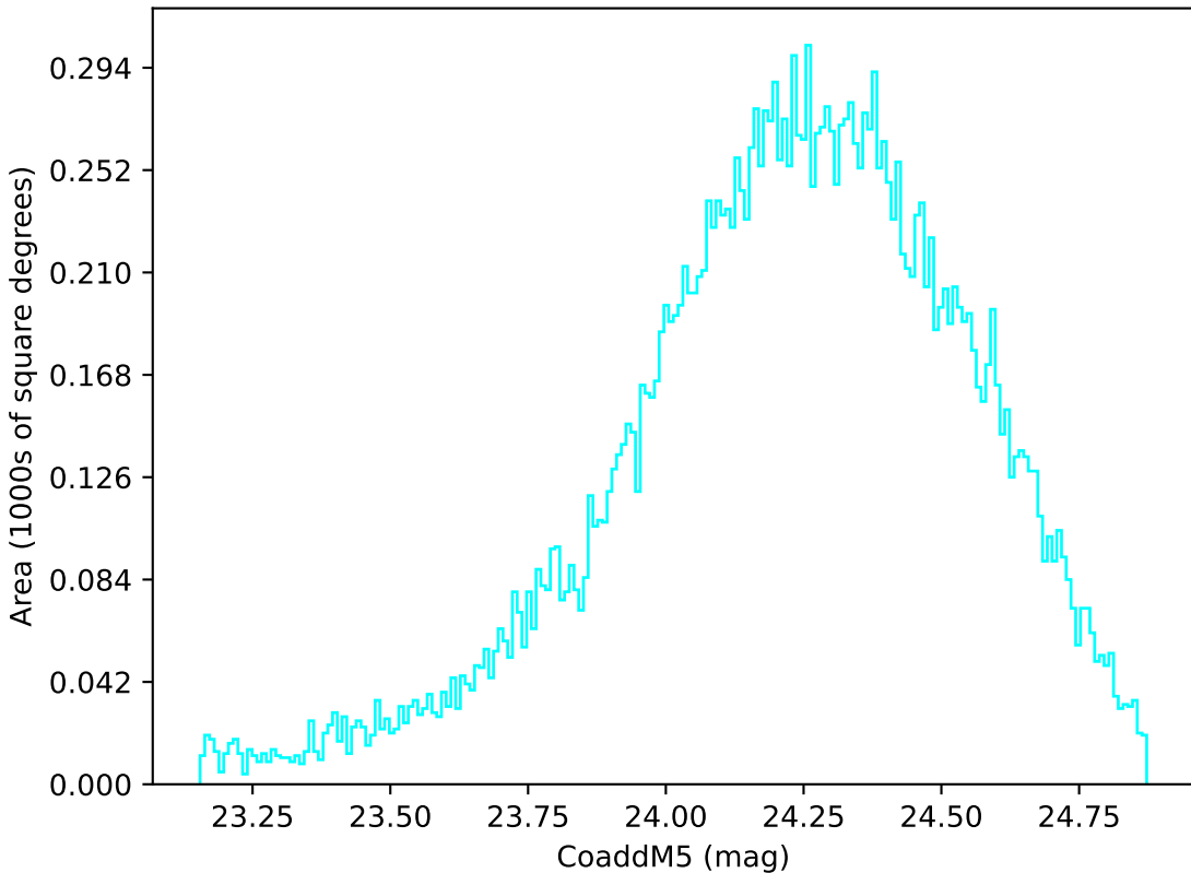
too_combined_s0.5_v3.4_10yrs Yr 1 u band: CoaddM5
