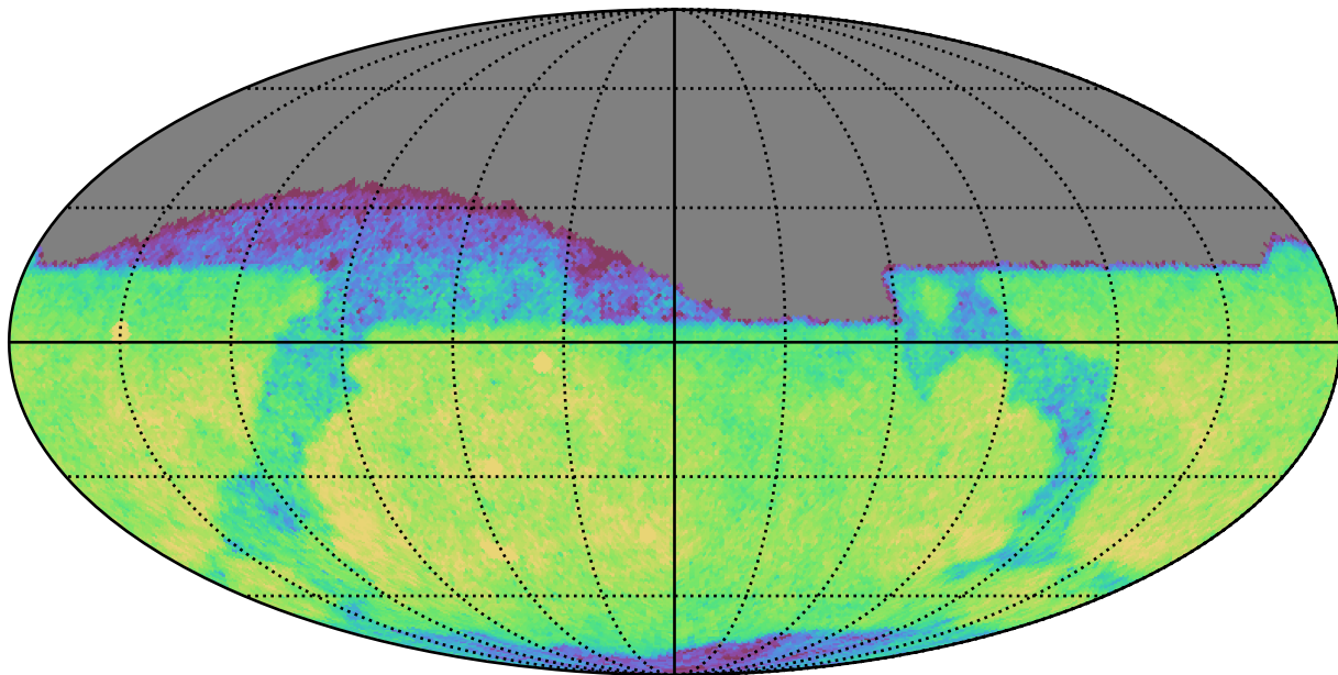
too_combined_s0.5_v3.4_10yrs Yr 1 r band: CoaddM5
