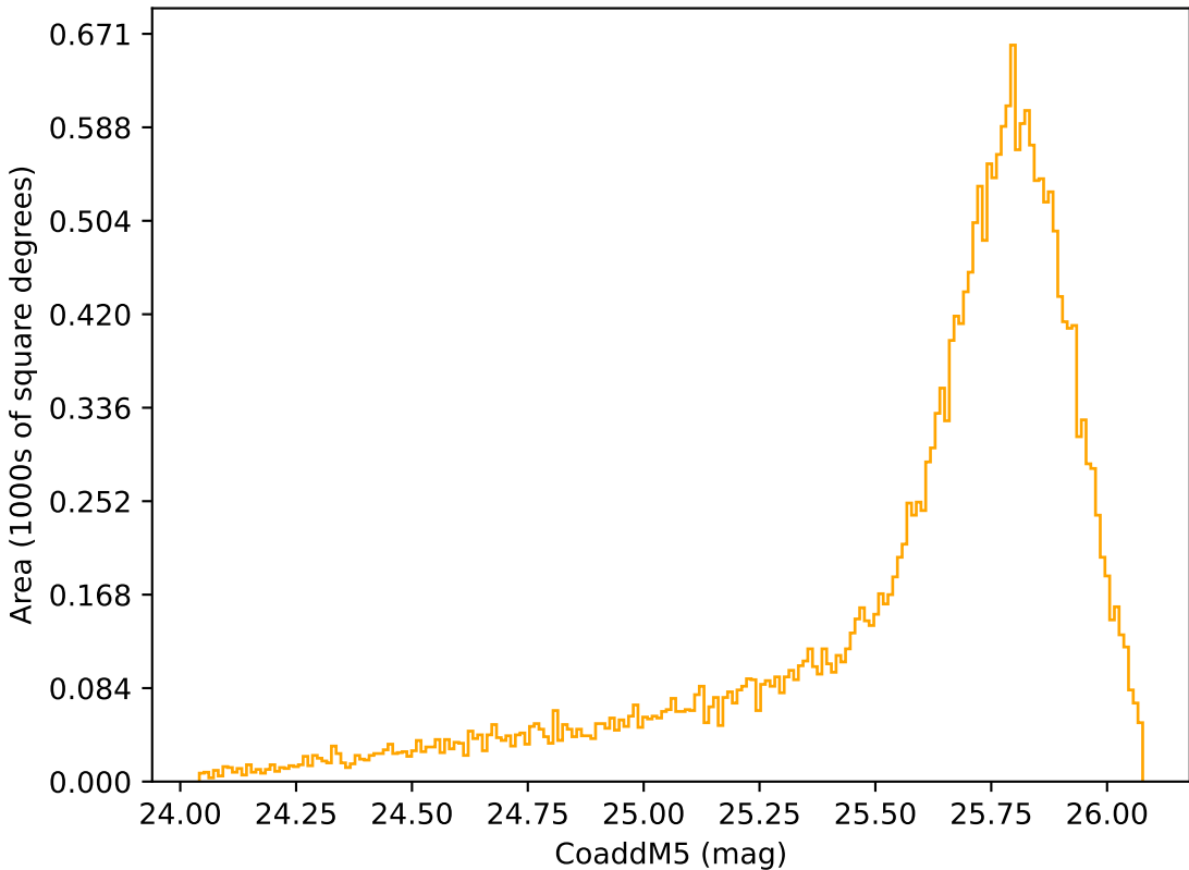
too_combined_s0.5_v3.4_10yrs Yr 1 r band: CoaddM5
