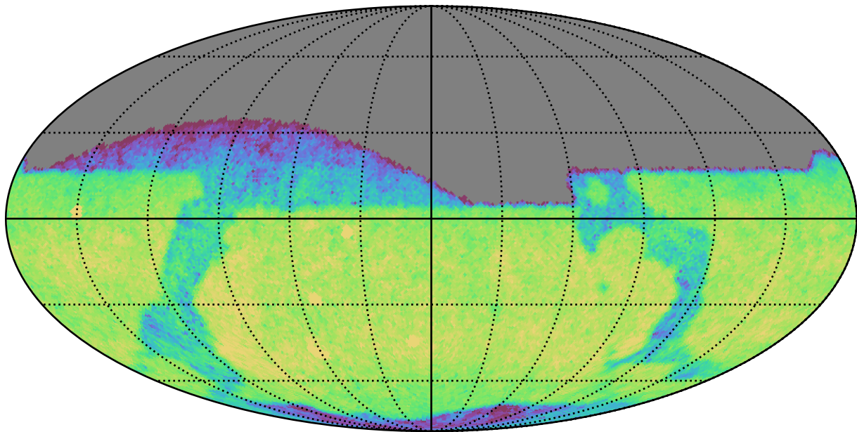
too_combined_s0.5_v3.4_10yrs Yr 1 i band: CoaddM5
