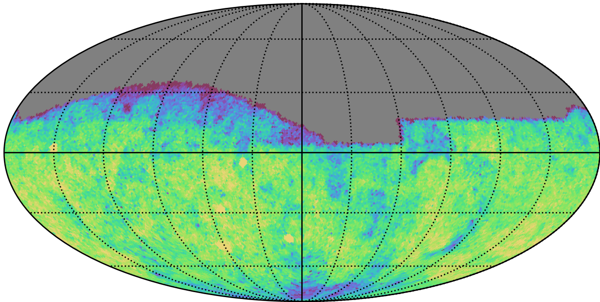
too_combined_s0.5_v3.4_10yrs Yr 1 g band: CoaddM5
