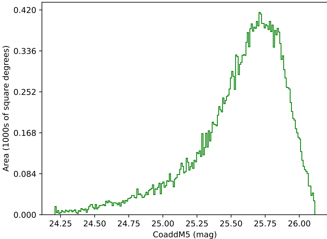
too_combined_s0.5_v3.4_10yrs Yr 1 g band: CoaddM5
