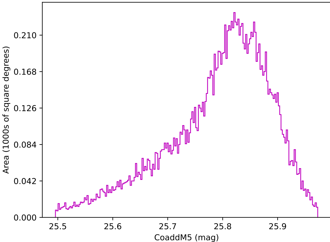
too_combined_s0.5_v3.4_10yrs WFD z band: CoaddM5
