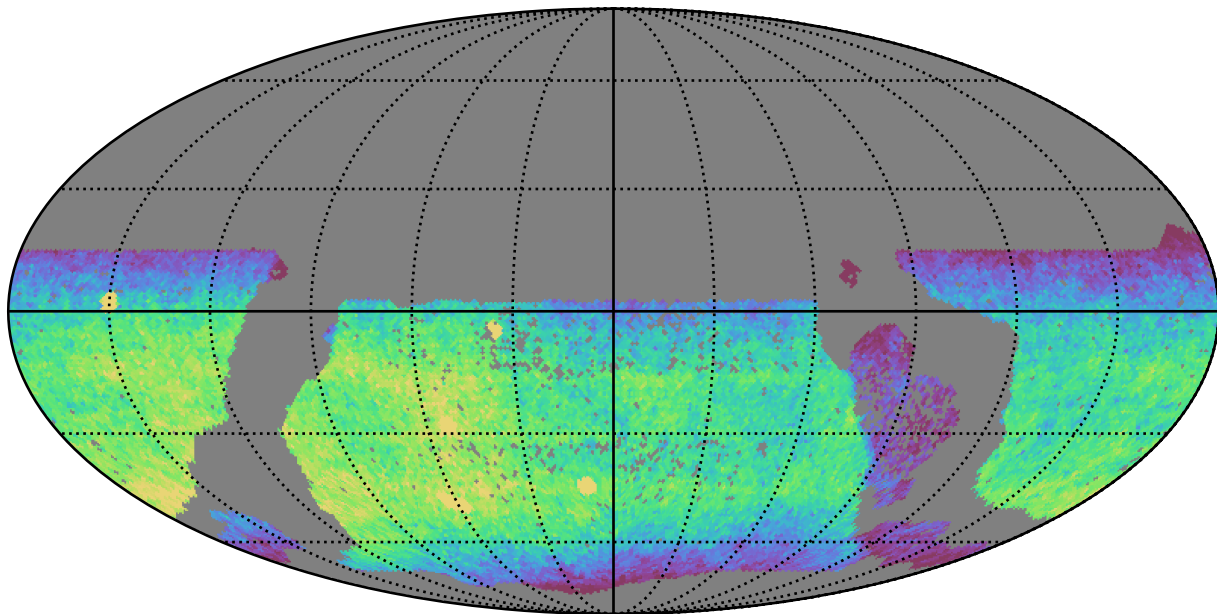
too_combined_s0.5_v3.4_10yrs WFD y band: CoaddM5
