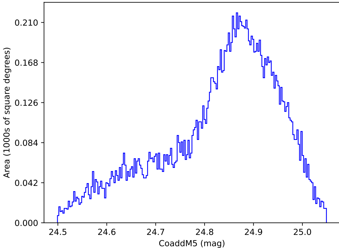
too_combined_s0.5_v3.4_10yrs WFD y band: CoaddM5
