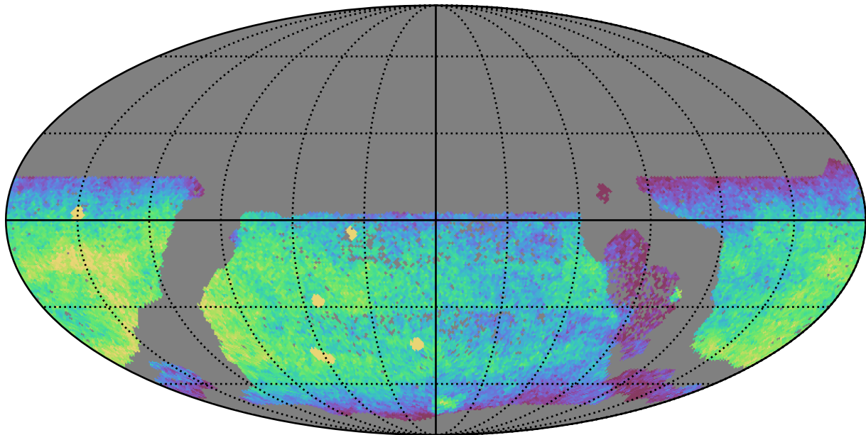
too_combined_s0.5_v3.4_10yrs WFD u band: CoaddM5
