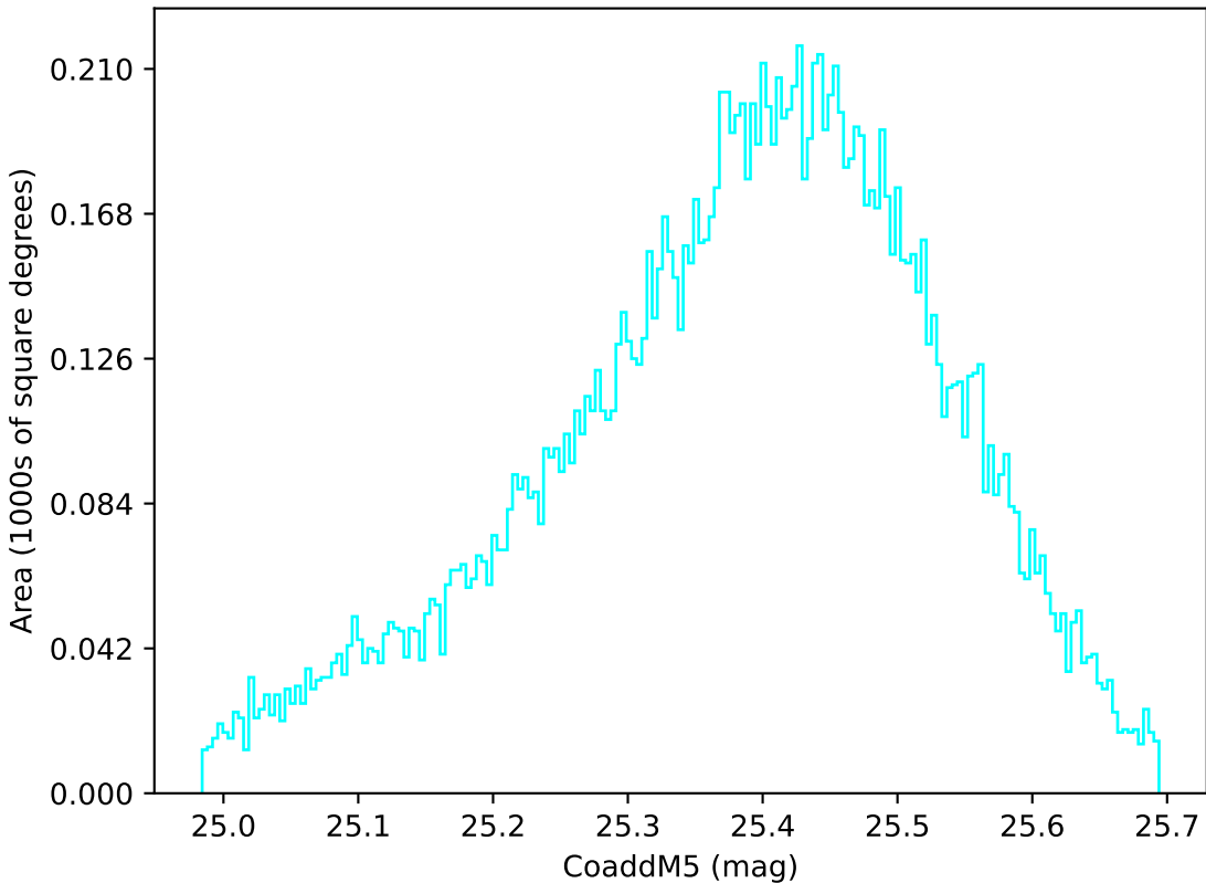
too_combined_s0.5_v3.4_10yrs WFD u band: CoaddM5
