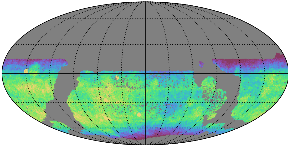
too_combined_s0.5_v3.4_10yrs WFD i band: CoaddM5
