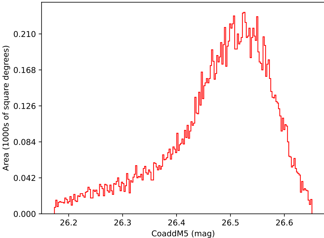
too_combined_s0.5_v3.4_10yrs WFD i band: CoaddM5
