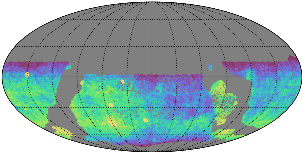
too_combined_s0.5_v3.4_10yrs WFD g band: CoaddM5
