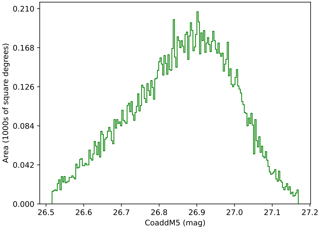
too_combined_s0.5_v3.4_10yrs WFD g band: CoaddM5
