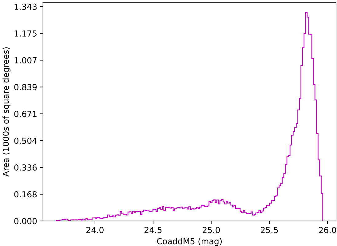
too_combined_s0.5_v3.4_10yrs All sky z band: CoaddM5
