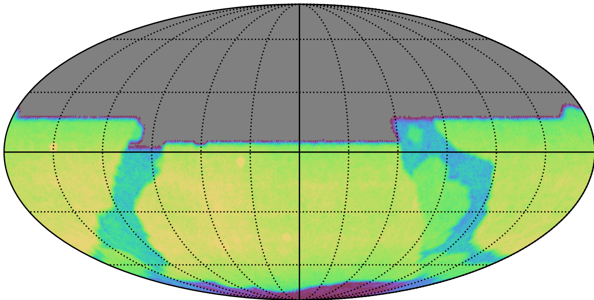
too_combined_s0.5_v3.4_10yrs All sky y band: CoaddM5
