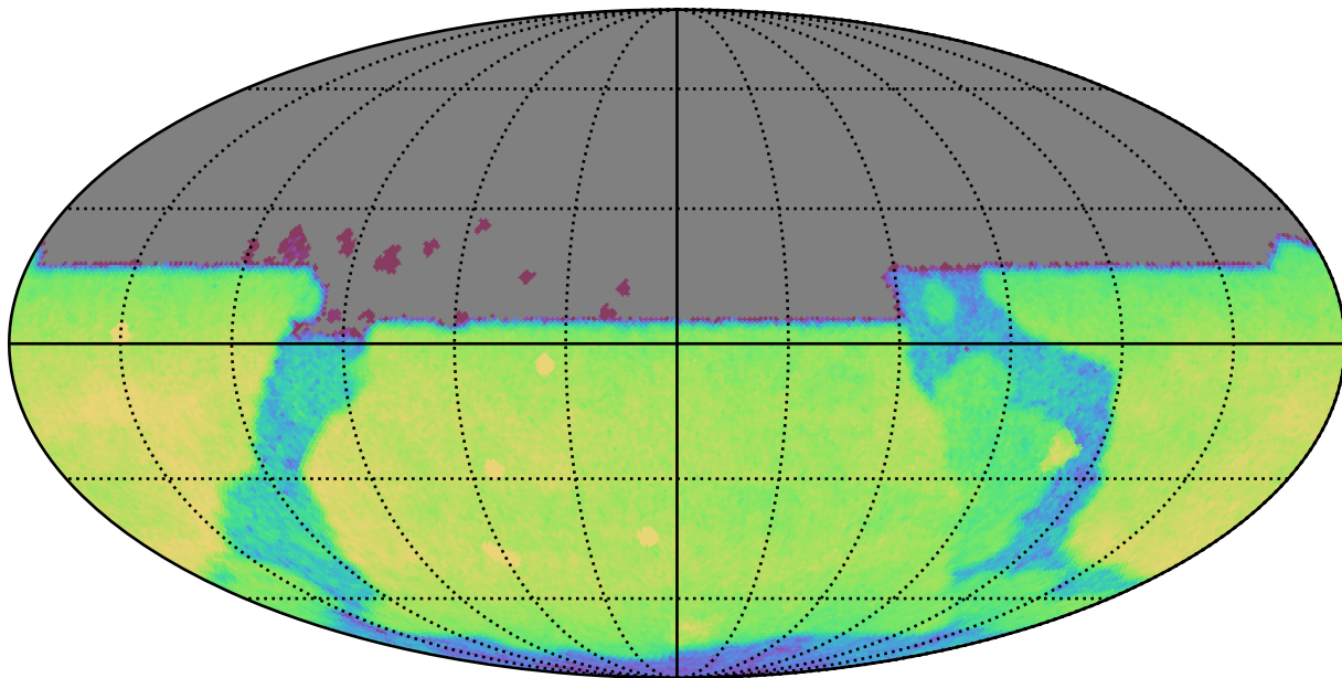
too_combined_s0.5_v3.4_10yrs All sky u band: CoaddM5
