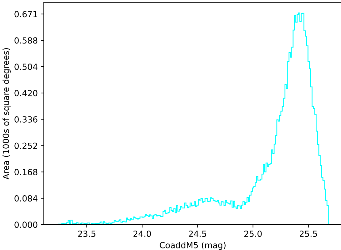
too_combined_s0.5_v3.4_10yrs All sky u band: CoaddM5
