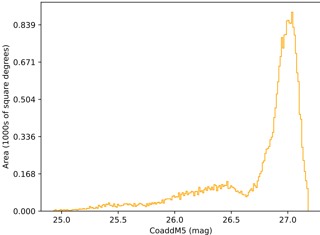
too_combined_s0.5_v3.4_10yrs All sky r band: CoaddM5
