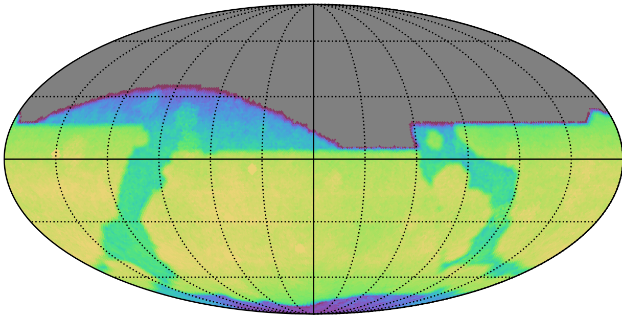
too_combined_s0.5_v3.4_10yrs All sky i band: CoaddM5
