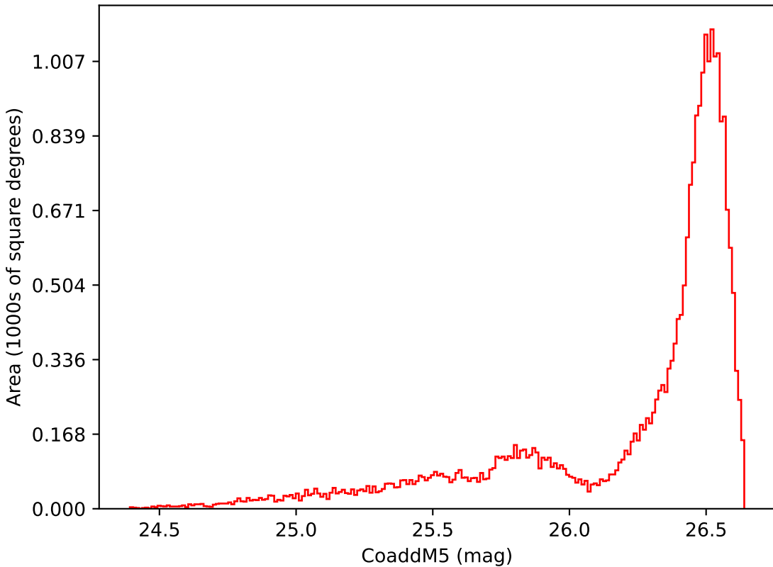
too_combined_s0.5_v3.4_10yrs All sky i band: CoaddM5
