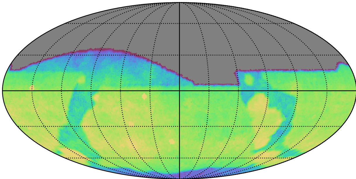
too_combined_s0.5_v3.4_10yrs All sky g band: CoaddM5
