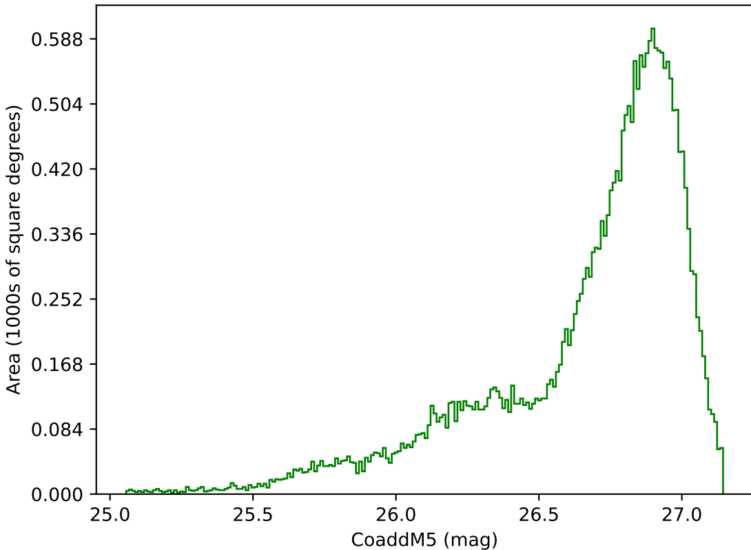
too_combined_s0.5_v3.4_10yrs All sky g band: CoaddM5
