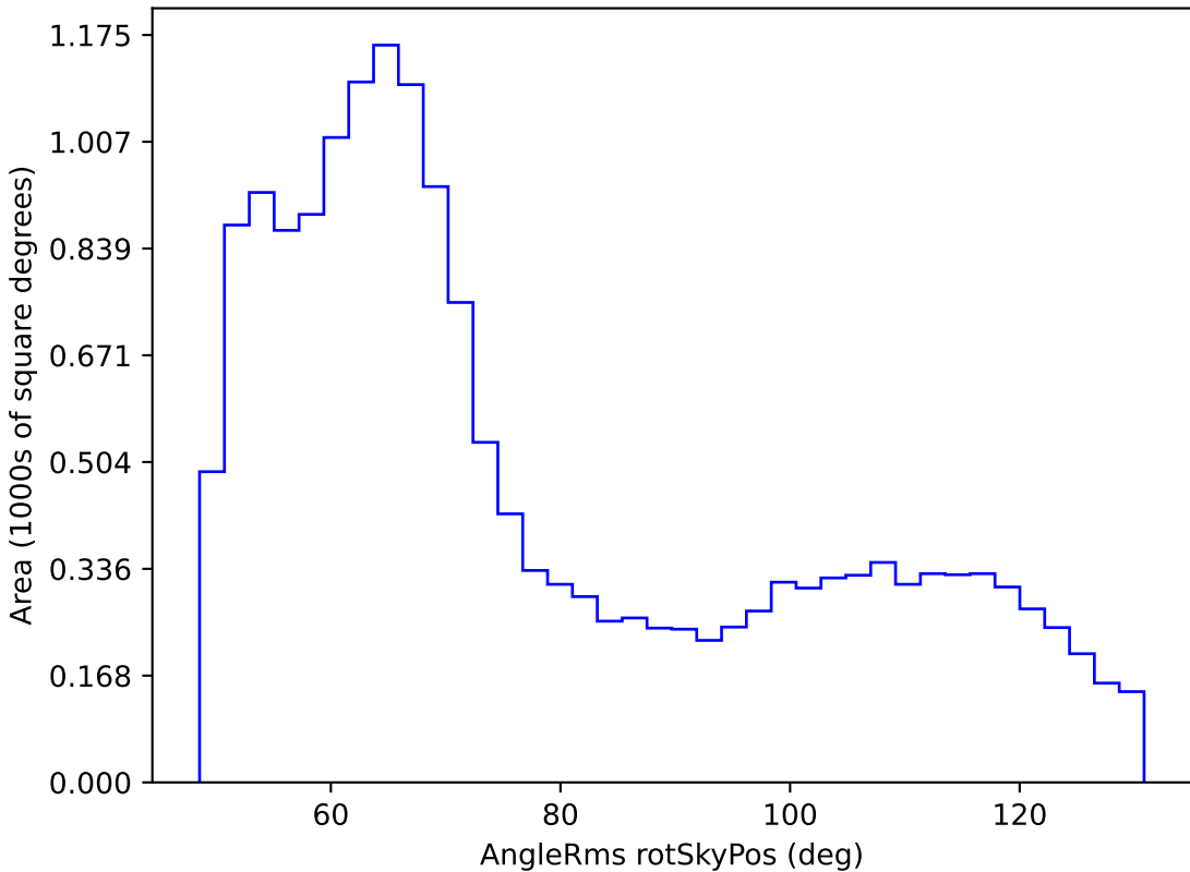
too_combined_s0.5_v3.4_10yrs WFD z band: AngleRms rotSkyPos
