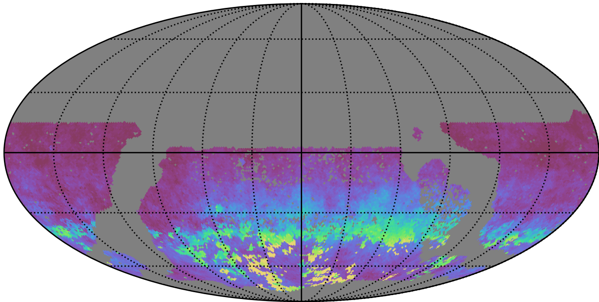
too_combined_s0.5_v3.4_10yrs WFD y band: AngleRms rotSkyPos
