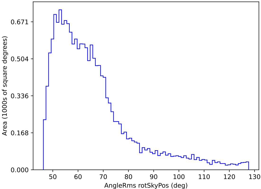
too_combined_s0.5_v3.4_10yrs WFD y band: AngleRms rotSkyPos
