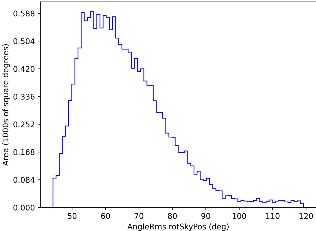
too_combined_s0.5_v3.4_10yrs WFD u band: AngleRms rotSkyPos
