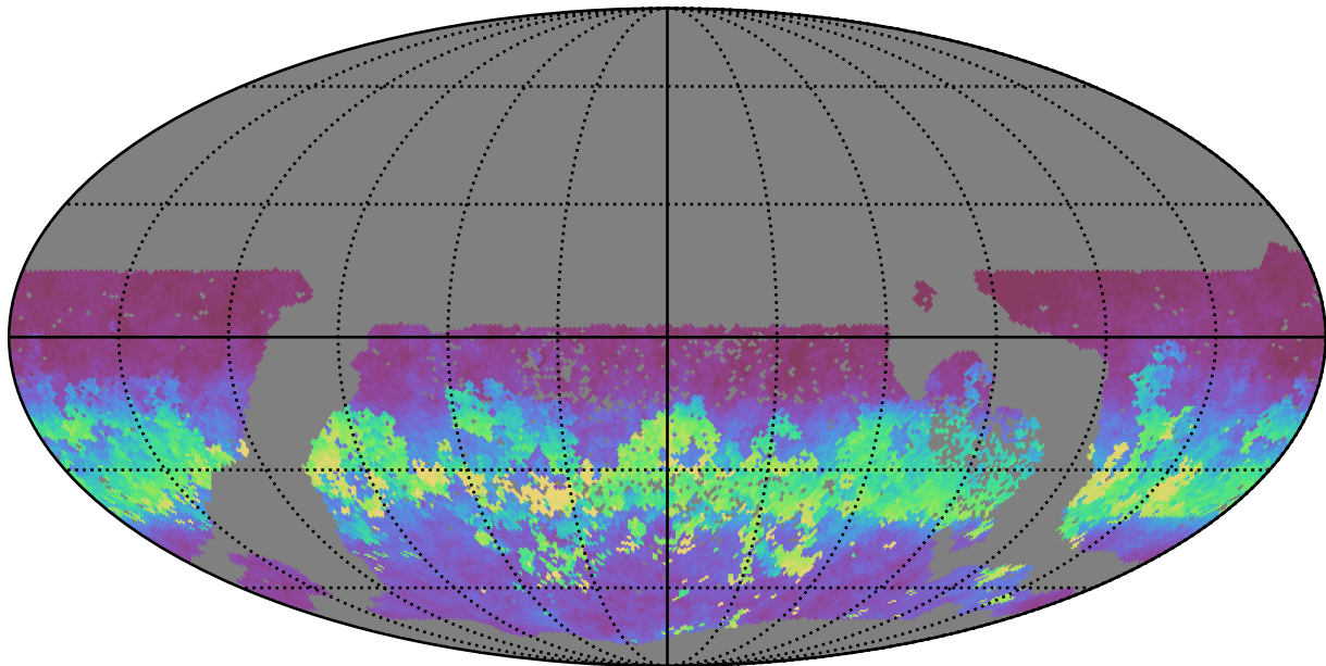
too_combined_s0.5_v3.4_10yrs WFD r band: AngleRms rotSkyPos
