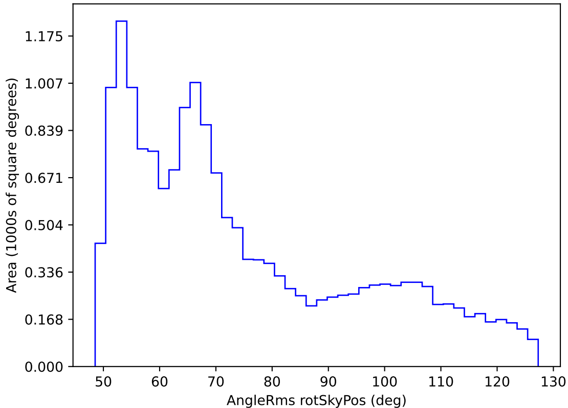
too_combined_s0.5_v3.4_10yrs WFD r band: AngleRms rotSkyPos
