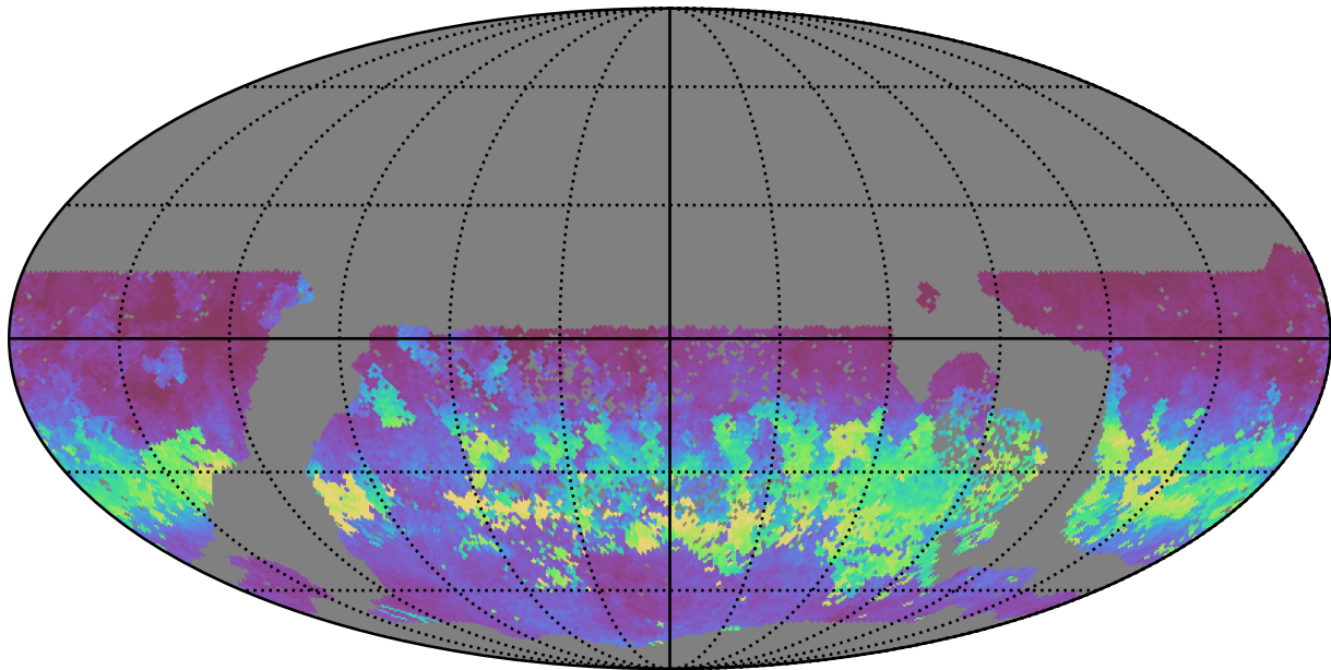
too_combined_s0.5_v3.4_10yrs WFD i band: AngleRms rotSkyPos
