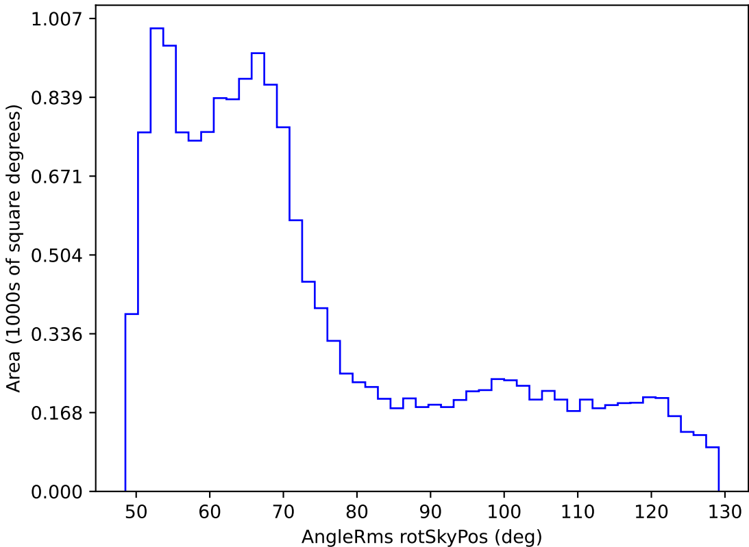
too_combined_s0.5_v3.4_10yrs WFD i band: AngleRms rotSkyPos
