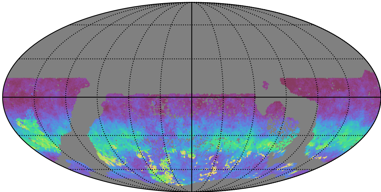
too_combined_s0.5_v3.4_10yrs WFD g band: AngleRms rotSkyPos
