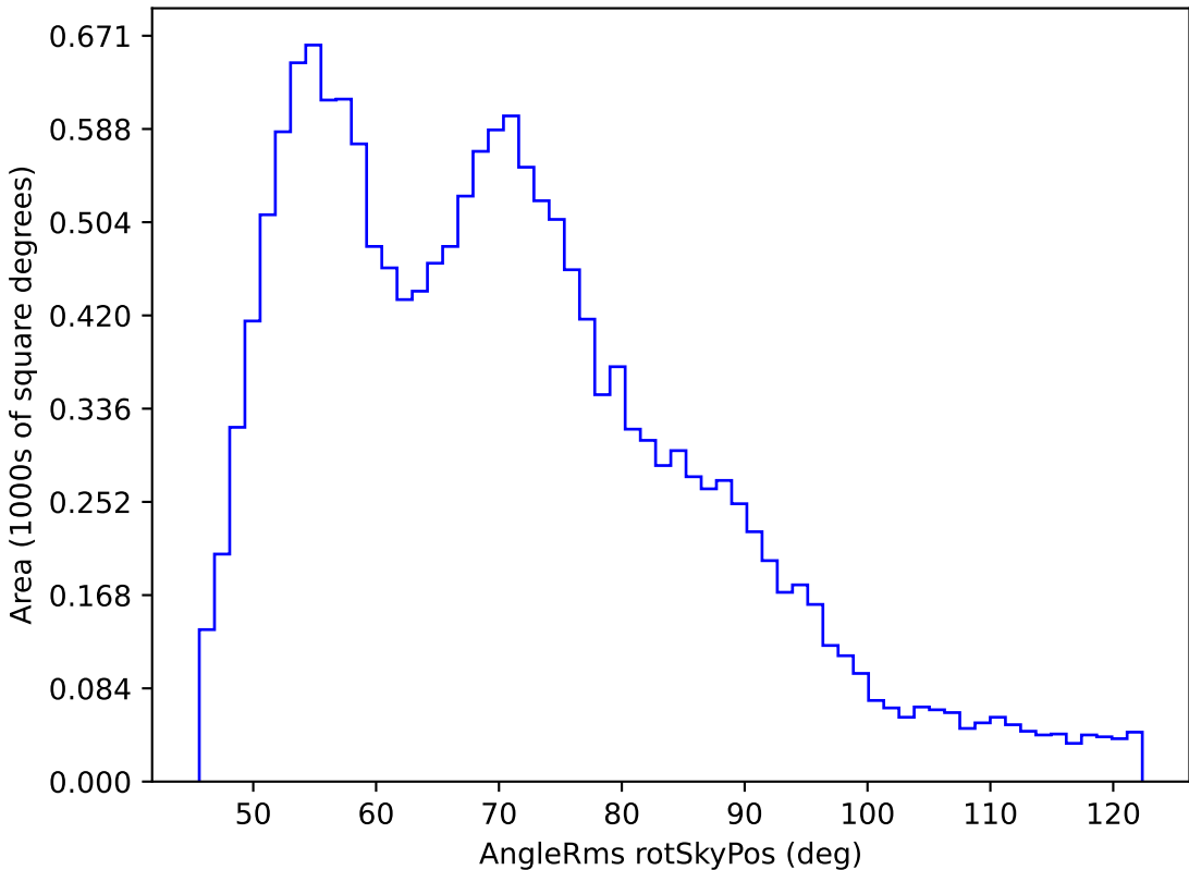
too_combined_s0.5_v3.4_10yrs WFD g band: AngleRms rotSkyPos
