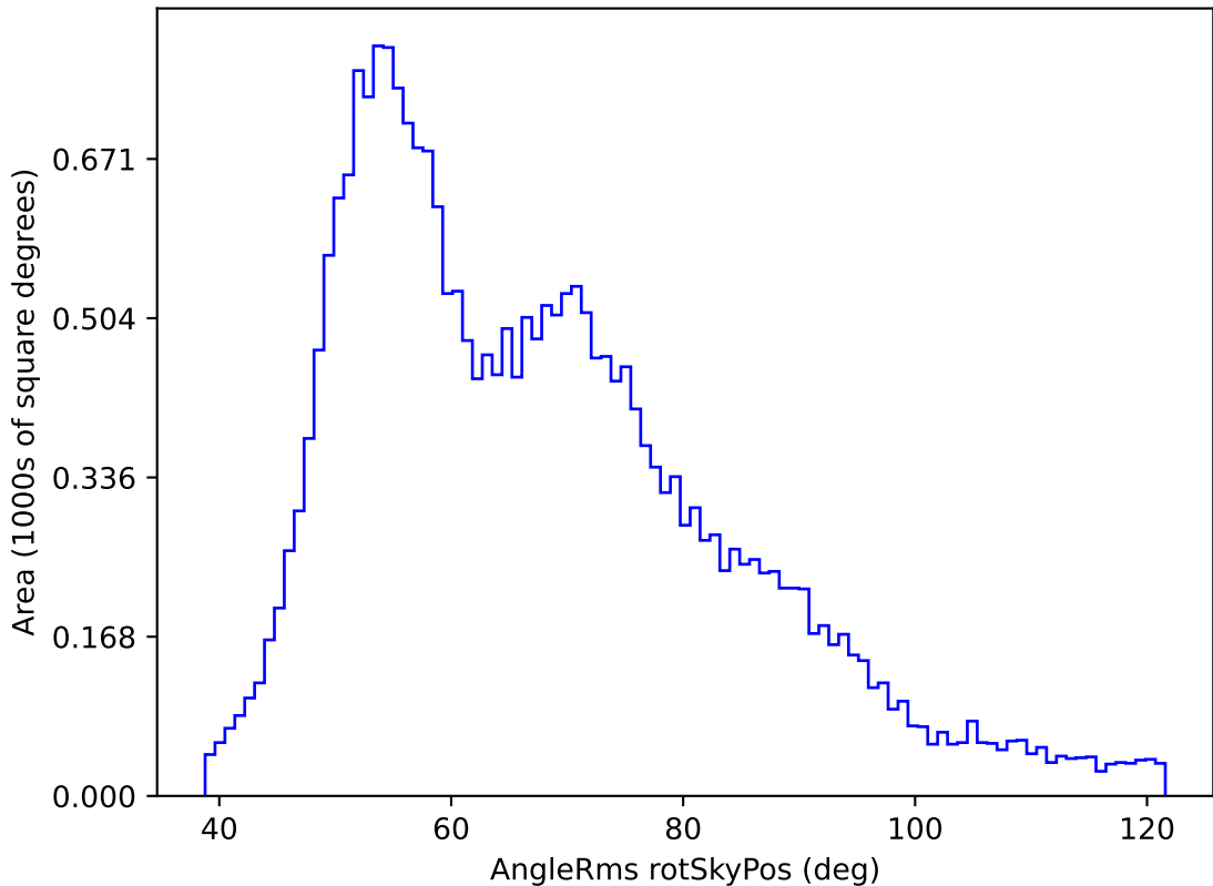
too_combined_s0.5_v3.4_10yrs All sky g band: AngleRms rotSkyPos
