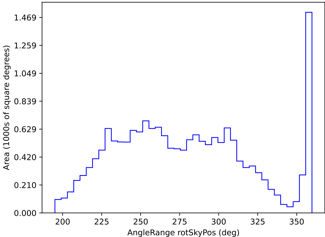
too_combined_s0.5_v3.4_10yrs WFD y band: AngleRange rotSkyPos
