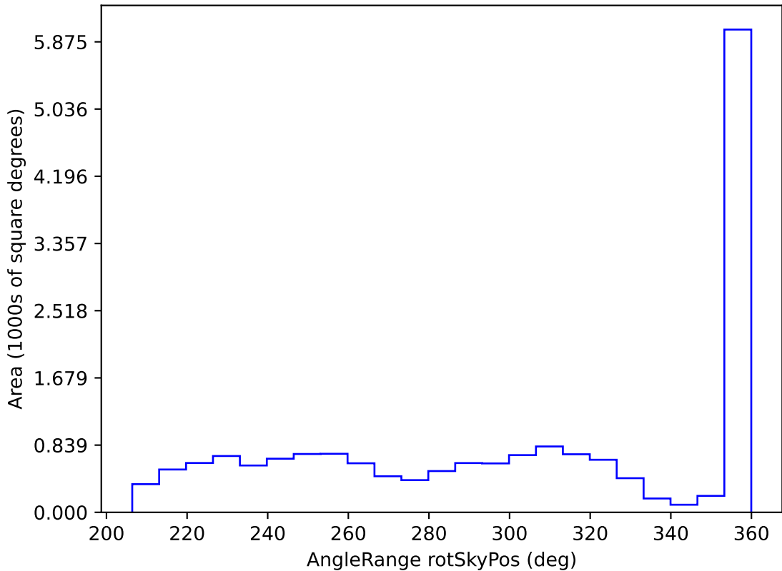
too_combined_s0.5_v3.4_10yrs WFD r band: AngleRange rotSkyPos
