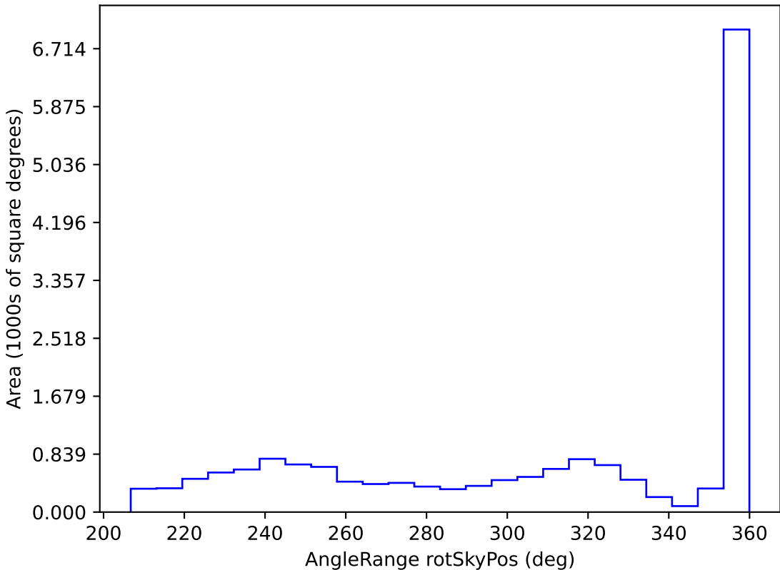
too_combined_s0.5_v3.4_10yrs WFD i band: AngleRange rotSkyPos
