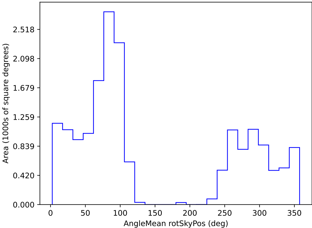
too_combined_s0.5_v3.4_10yrs WFD u band: AngleMean rotSkyPos
