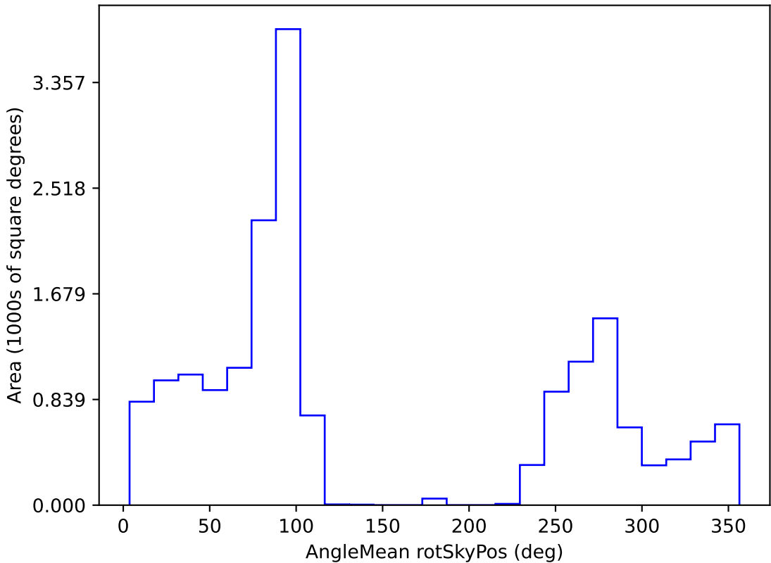
too_combined_s0.5_v3.4_10yrs WFD r band: AngleMean rotSkyPos
