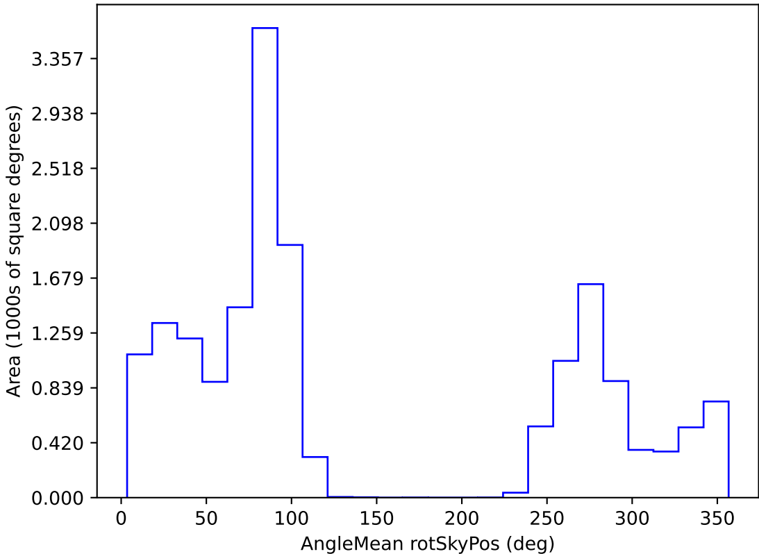
too_combined_s0.5_v3.4_10yrs WFD i band: AngleMean rotSkyPos
