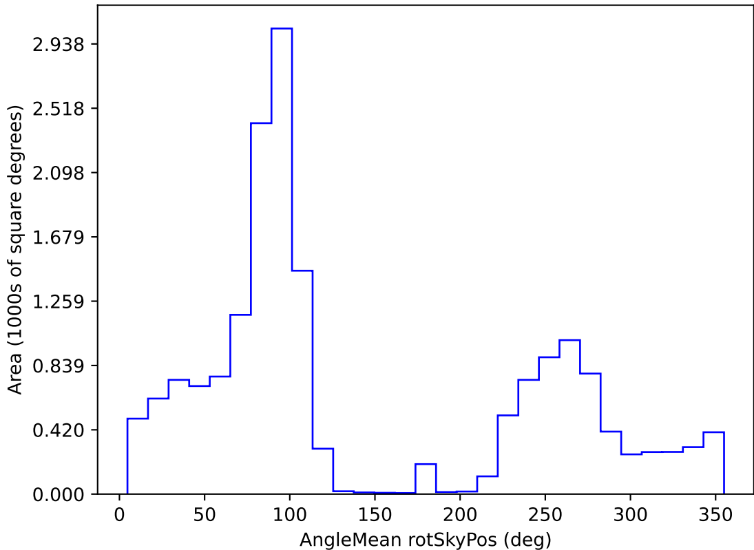
too_combined_s0.5_v3.4_10yrs WFD g band: AngleMean rotSkyPos
