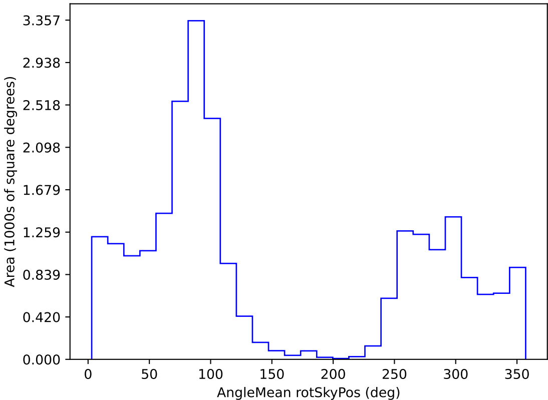
too_combined_s0.5_v3.4_10yrs All sky u band: AngleMean rotSkyPos
