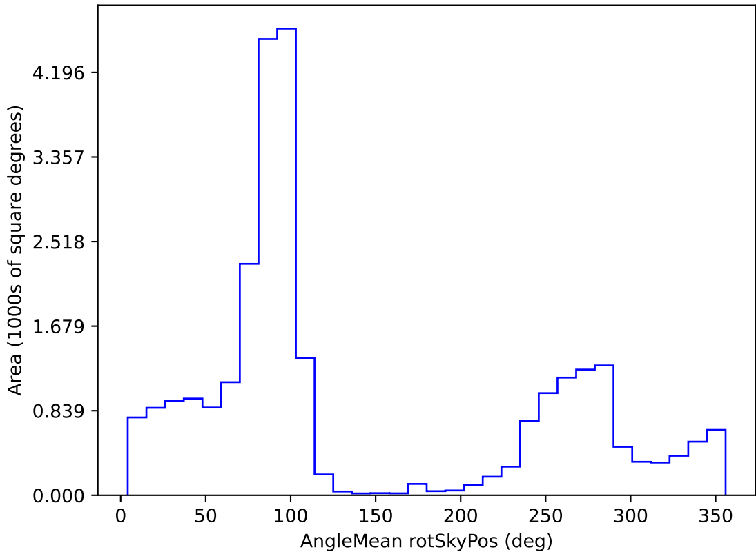
too_combined_s0.5_v3.4_10yrs All sky r band: AngleMean rotSkyPos
